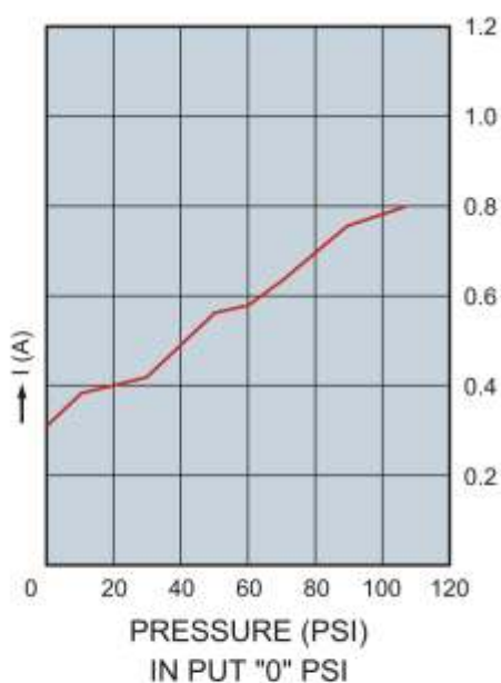
CURRENT CURVE
