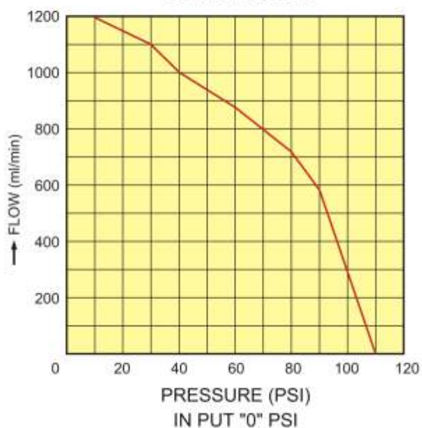
OUTLET CURVE
